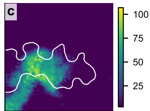
Clinical-memory prediction
